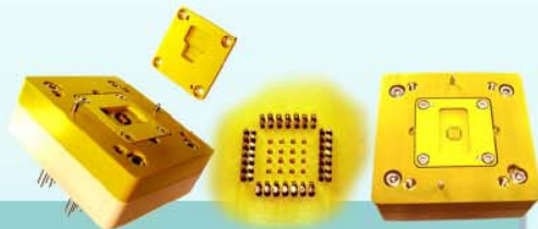
0.5mm Pitch Kelvin Test Socket for Multitest Handler (28L, MLP 5 x 5mm)
